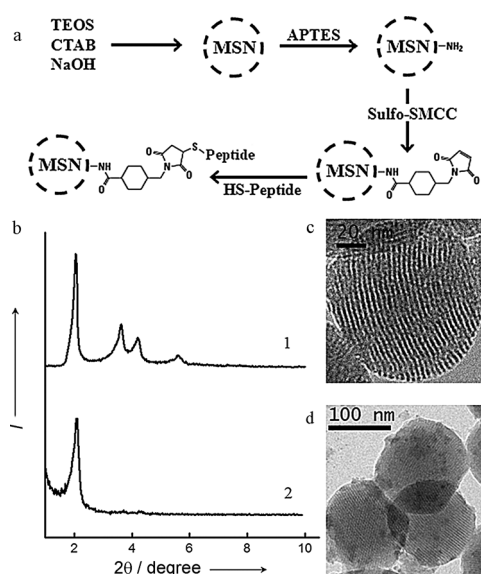
Figure 1. a) Strategies for MSN functionalized with peptide containing cysteine residue by using sulfo-SMCC. b) Small-angle XRD of MSNs (1) and Dox-loaded pHLIPss-MSNs (2); c) TEM image of naked MSNs; d) TEM image of Dox-loaded pHLIPss-MSNs.
